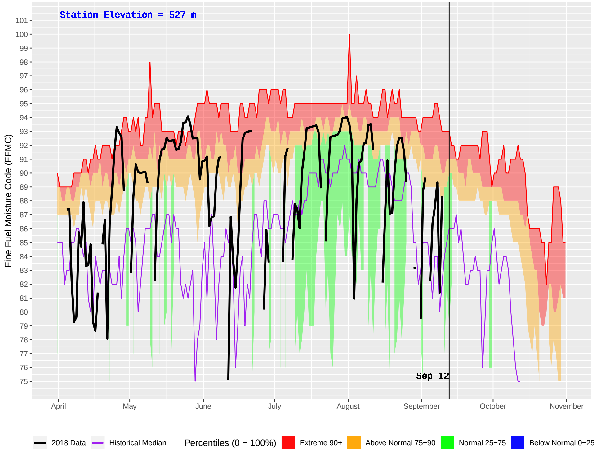
SALMON ARM (346) : Historical (1976–2016) and Current (2018) Daily Fine Fuel Moisture Code (FFMC)
