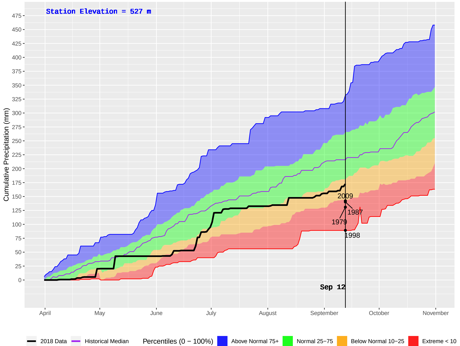
SALMON ARM (346) : Historical (1976–2016) and Current (2018) Daily Cumulative Precipitation
