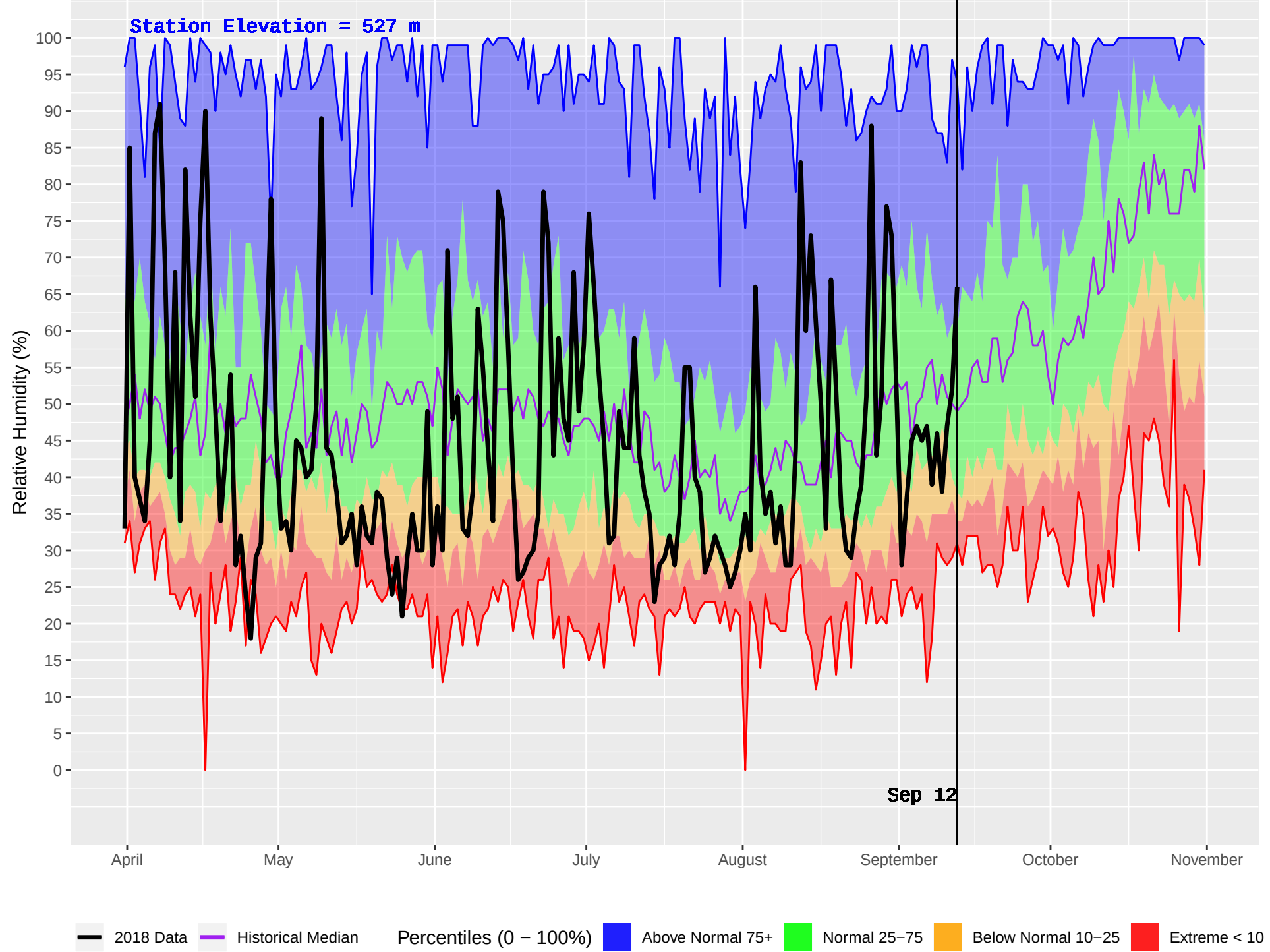
SALMON ARM (346) : Historical (1976–2016) and Current (2018) Daily Relative Humidity
