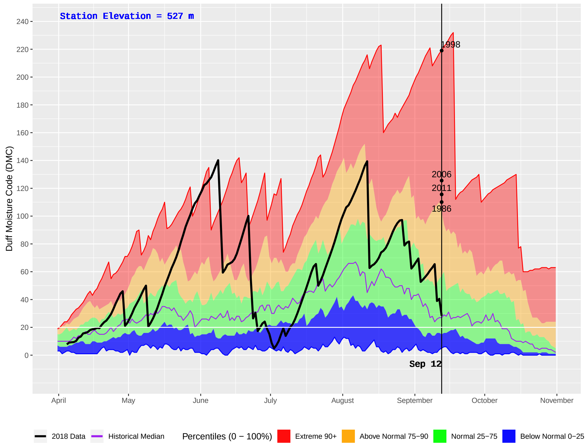
SALMON ARM (346) : Historical (1976–2016) and Current (2018) Daily Duff Moisture Code (DMC)
