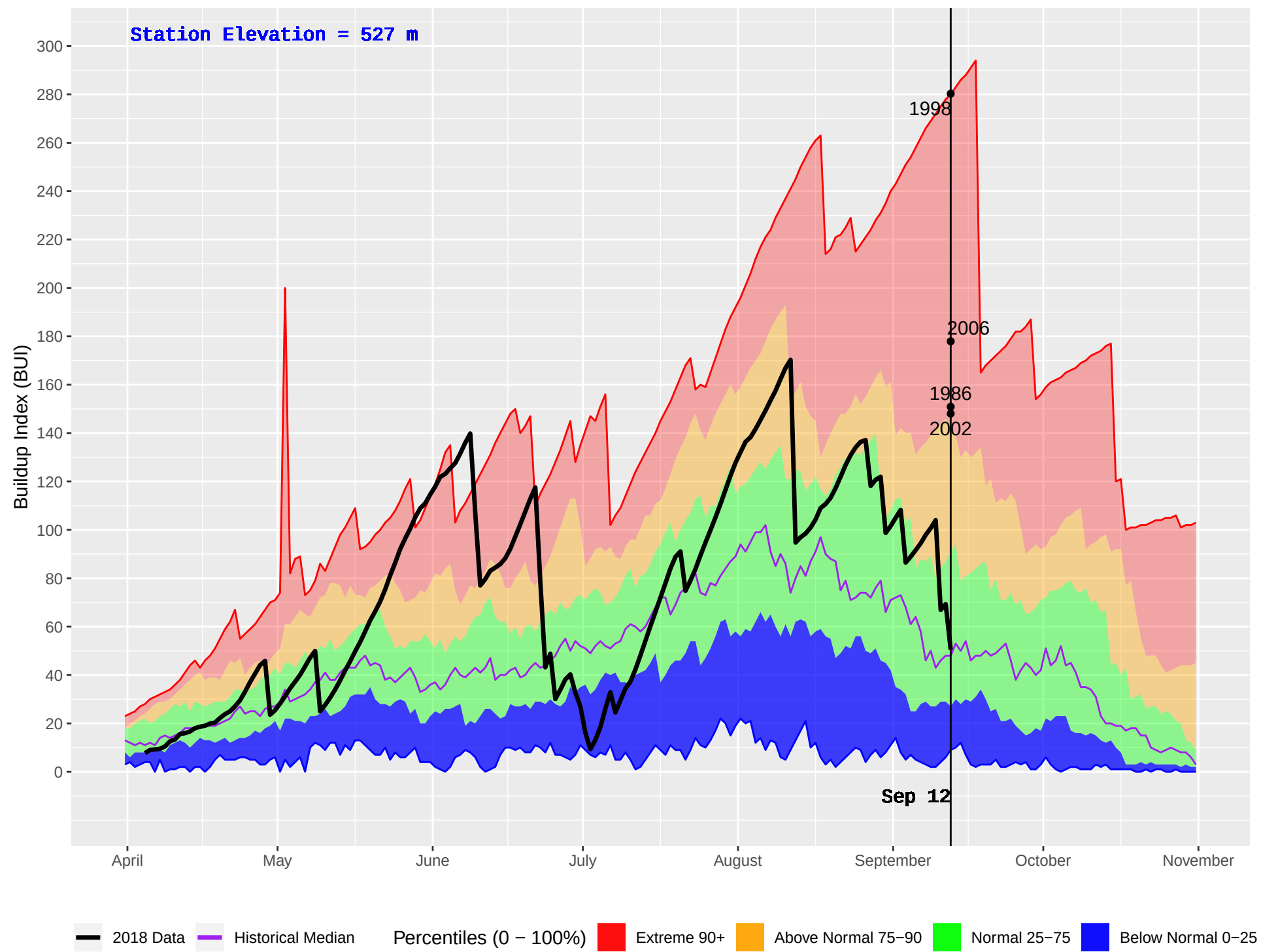
SALMON ARM (346) : Historical (1976–2016) and Current (2018) Daily Buildup Index (BUI)
