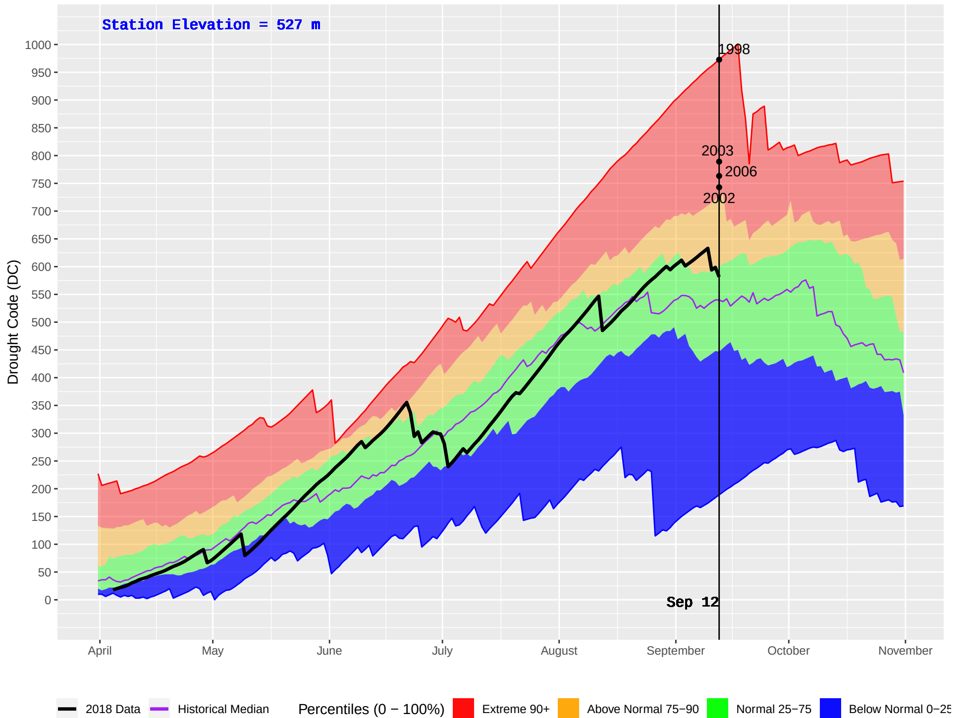
SALMON ARM (346) : Historical (1976–2016) and Current (2018) Daily Drought Code (DC)
